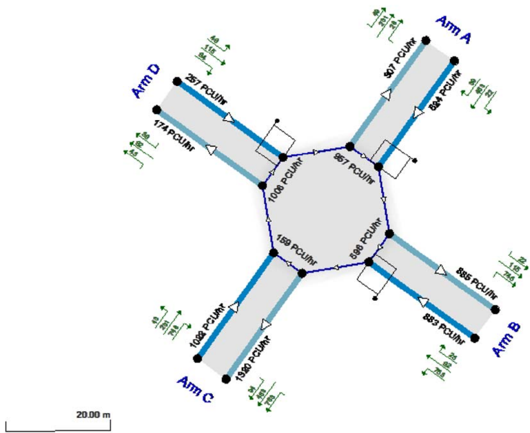
Showing modelled flow through junction (PCU/hr) Time Segment (06:45-07:00) Showing Analysis Set "A1 - Existing Layout"; Demand Set "D3 - 2022 - Future Year, AM" The junction diagram reflects the last run of ARCADY.
